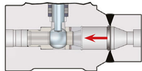
Socket weld end with nipple
