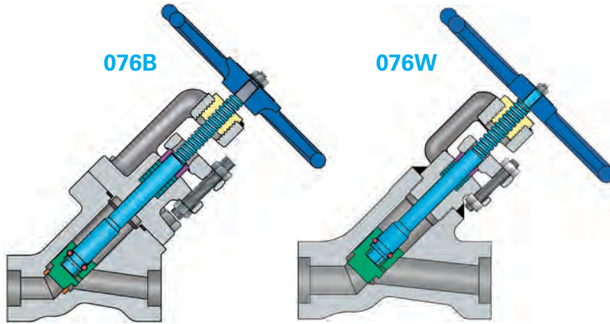
45° BOLTED BONNET
